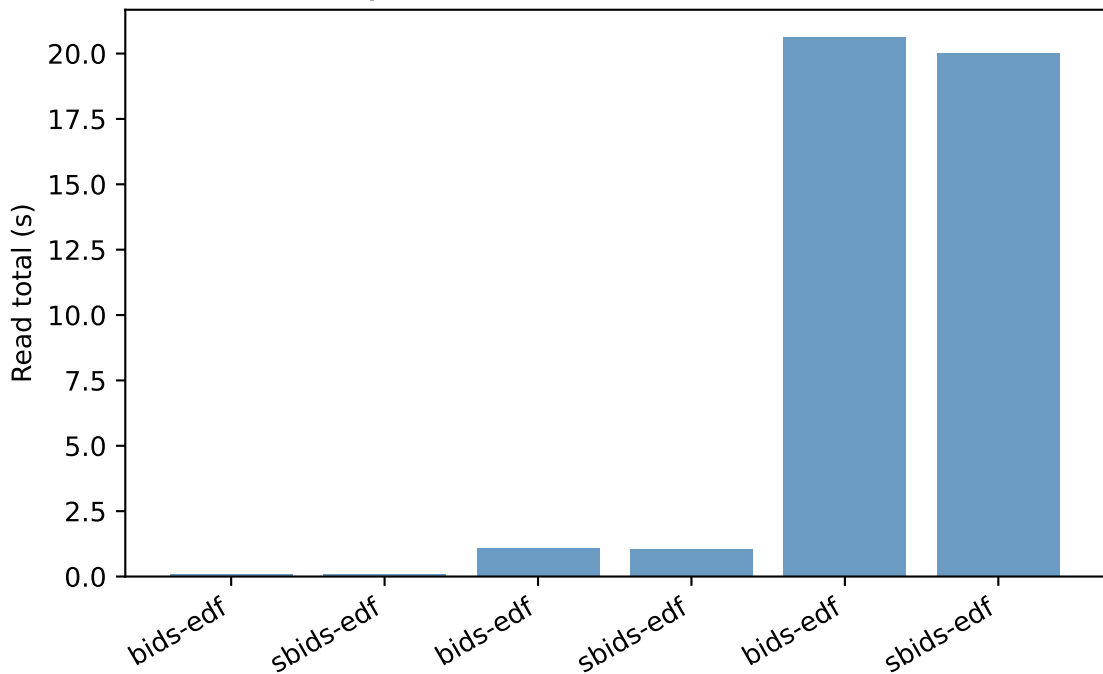
Synth format EDF – Read total (s)
