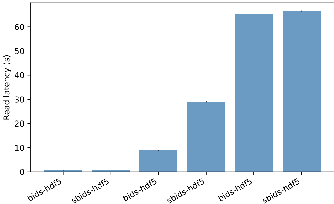
Synth format HDF5 - Read latency (s)
