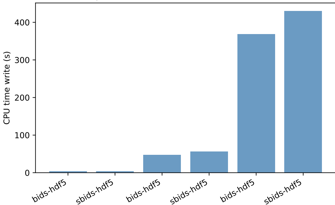
Synth format HDF5 - CPU time write (s)
