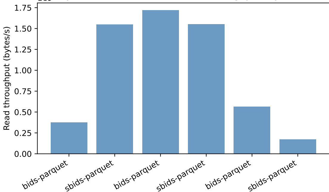
1e9 Synth format PARQUET - Read throughput (bytes/s)
