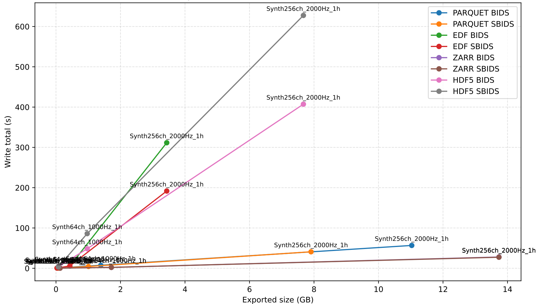
Synthetic datasets - Write total (s) vs size
