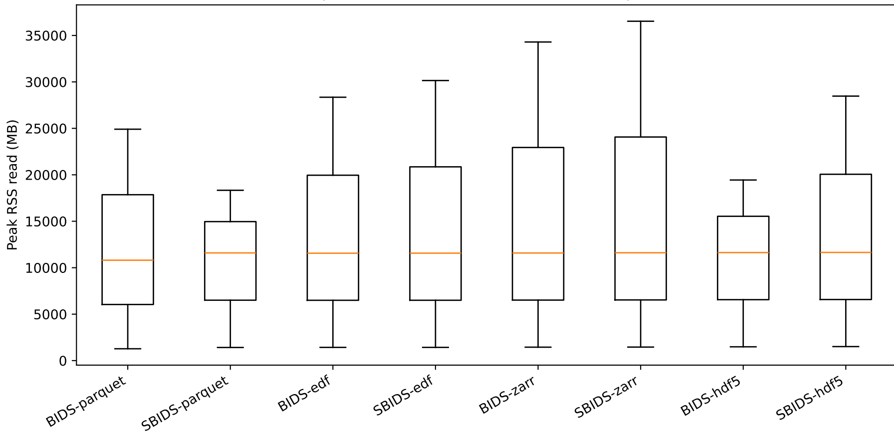
Experiment 2 - Peak RSS read (MB) (boxplots)
