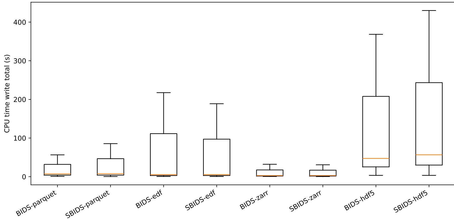
Experiment 2 - CPU time write total (s) (boxplots)
