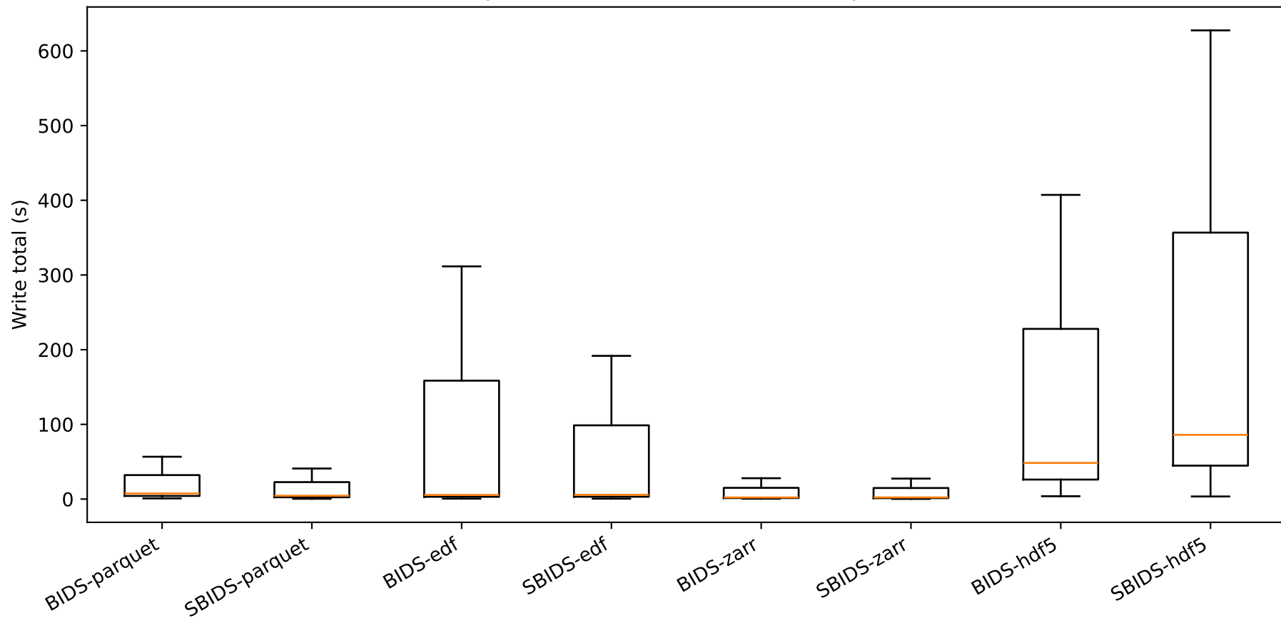
Experiment 2 - Write total (s) (boxplots)
