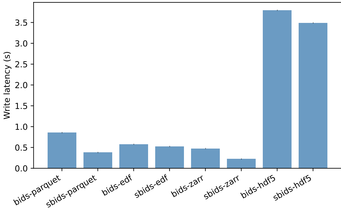
Synth Synth19ch_250Hz_1h - Write latency (s)
