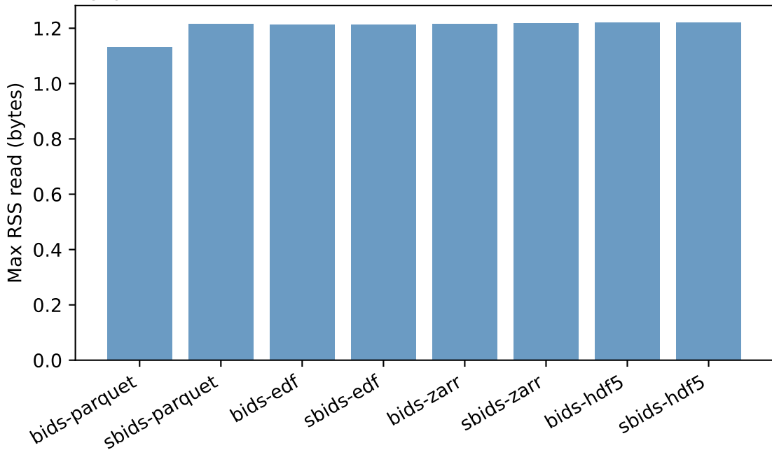
1e10 Synth Synth64ch_1000Hz_1h - Max RSS read (bytes)
