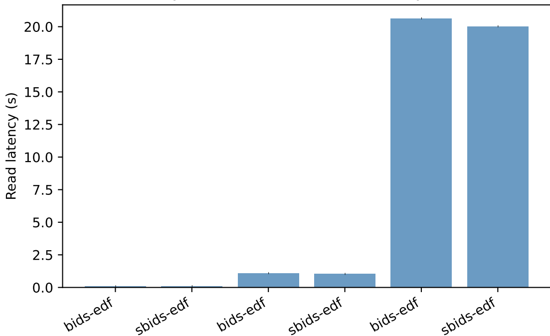
Synth format EDF – Read latency (s)
