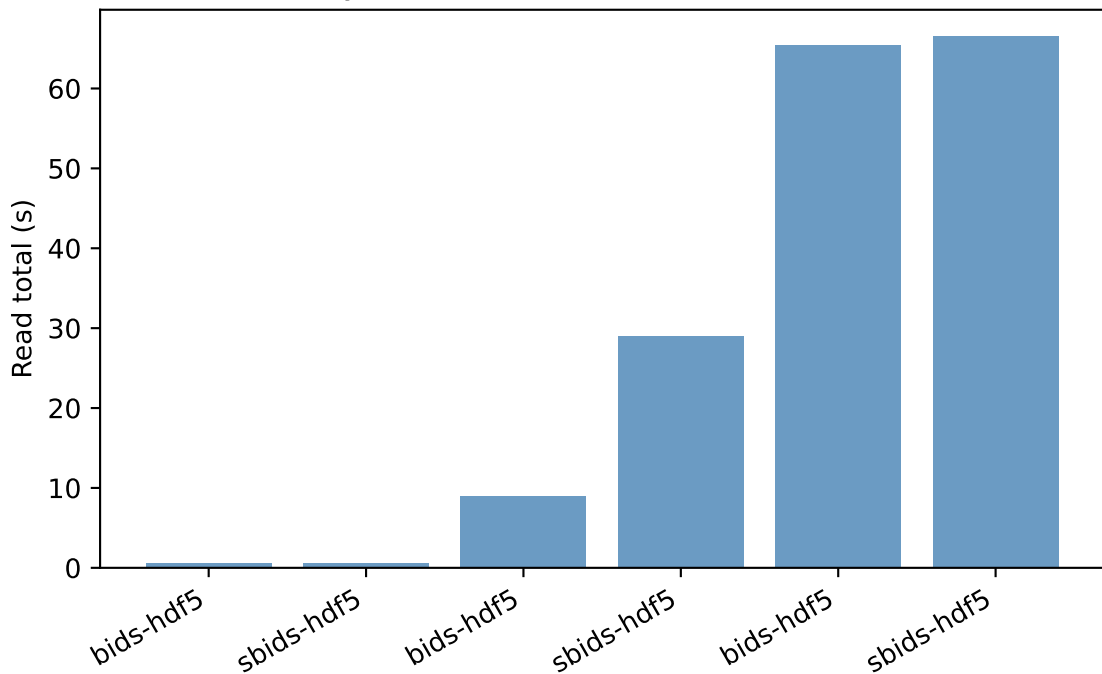
Synth format HDF5 - Read total (s)
