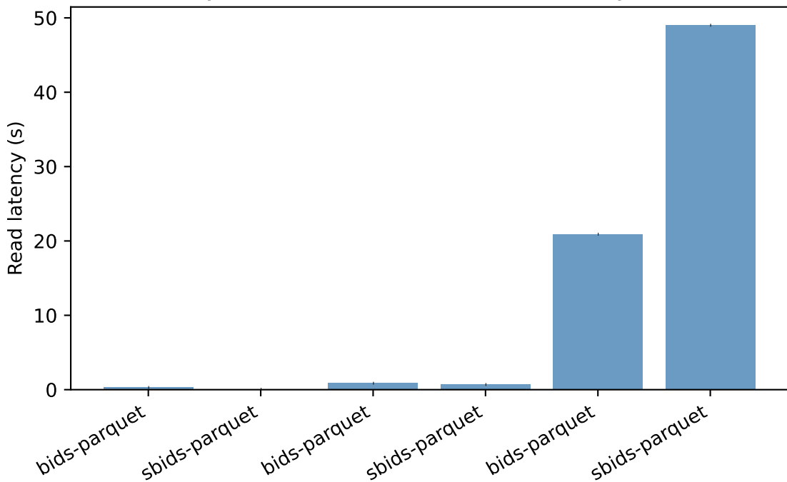
Synth format PARQUET - Read latency (s)
