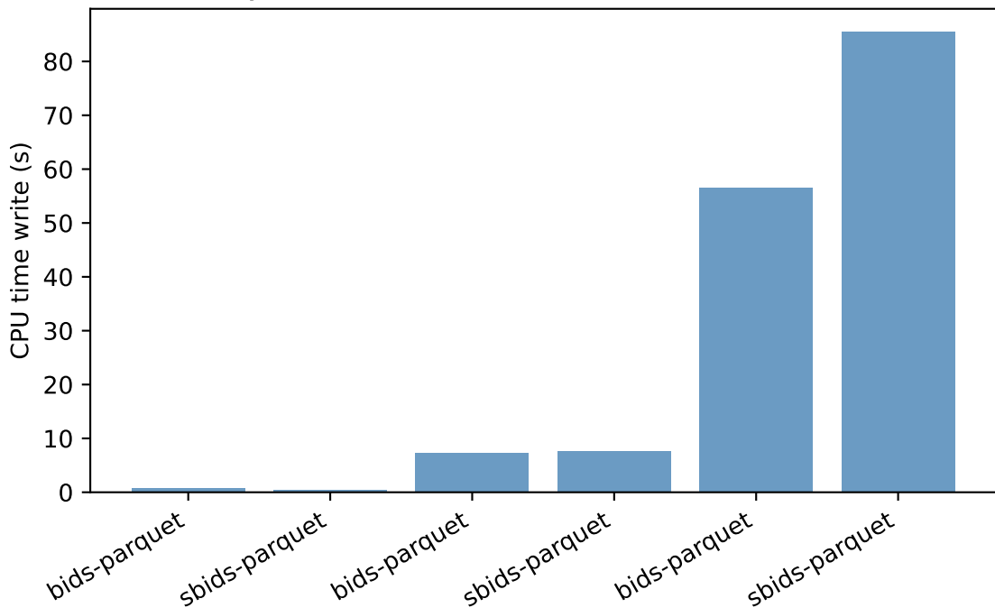
Synth format PARQUET - CPU time write (s)
