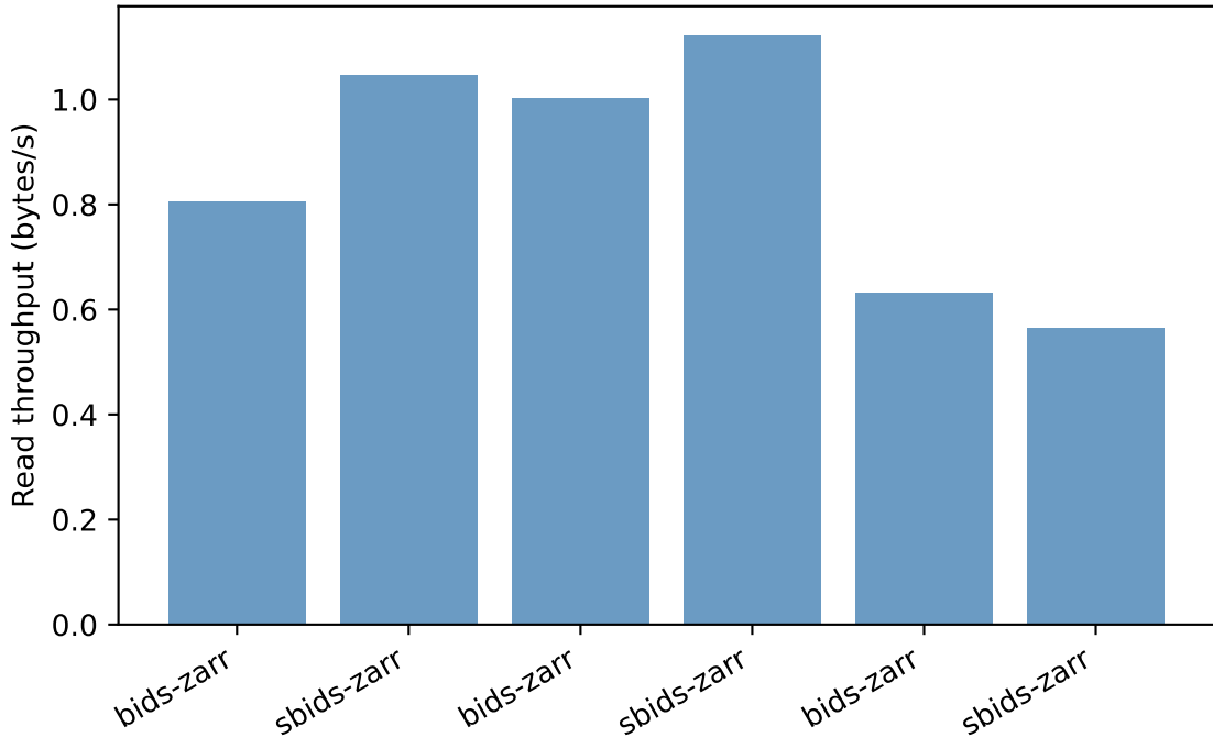
1e9 Synth format ZARR - Read throughput (bytes/s)
