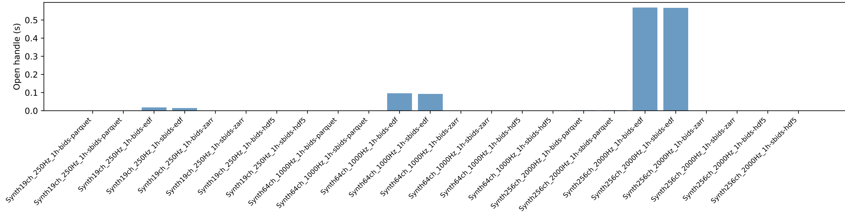
Streaming latency - Open handle (s)
