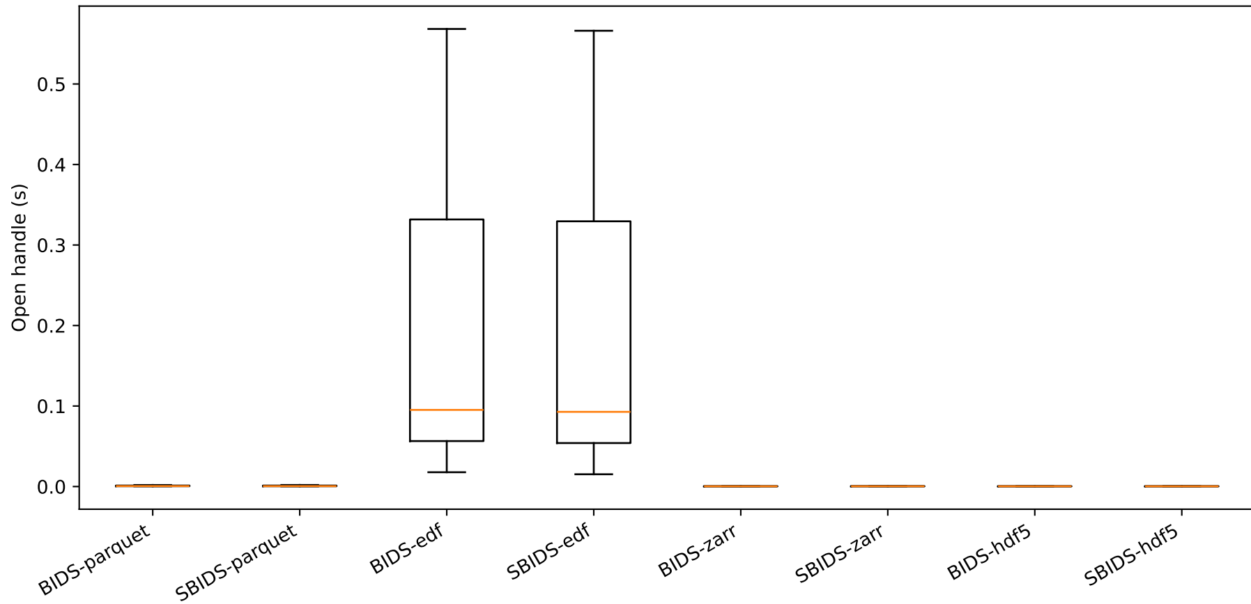
Streaming latency - Open handle (s) (boxplots)
