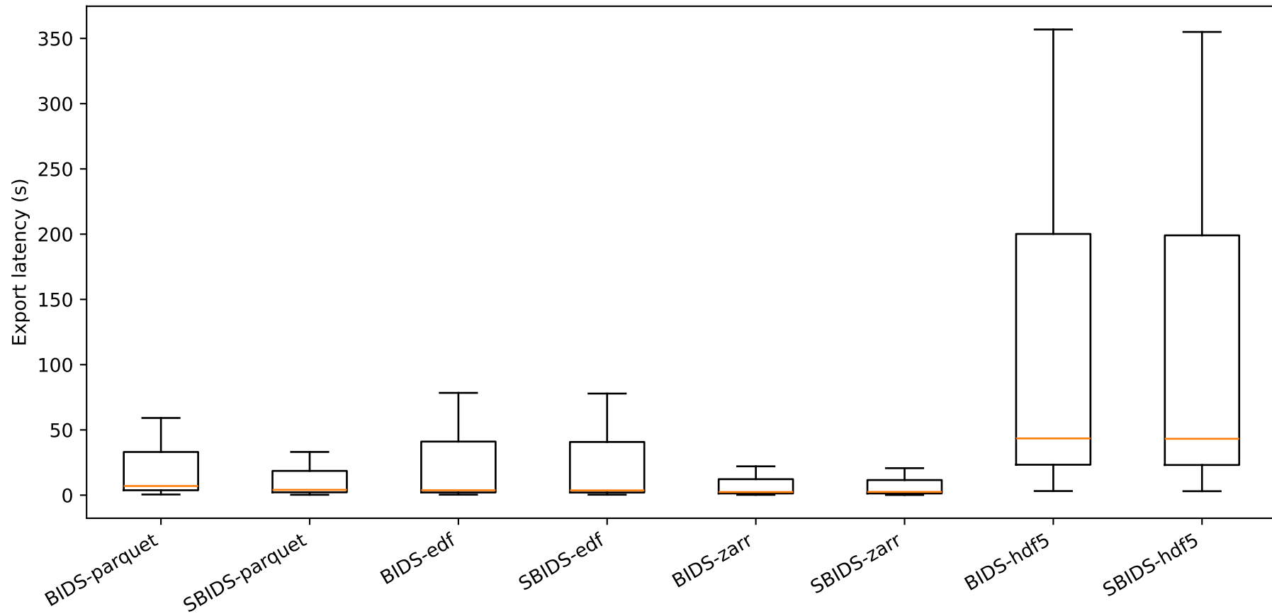
Write latency (export) by container/format
