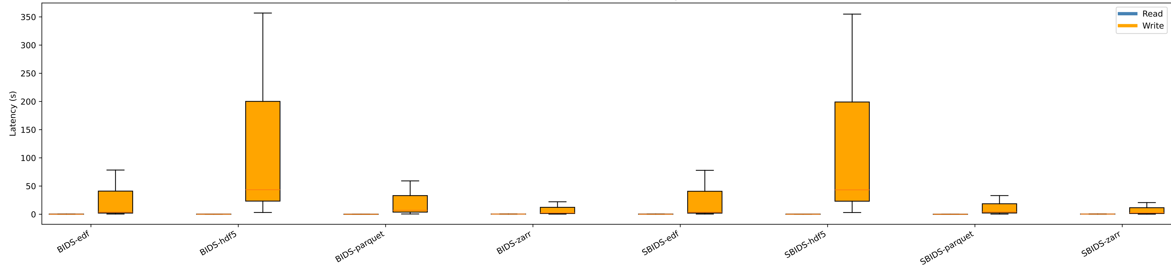
Read vs write latency (box) - Read full single channel (s)
