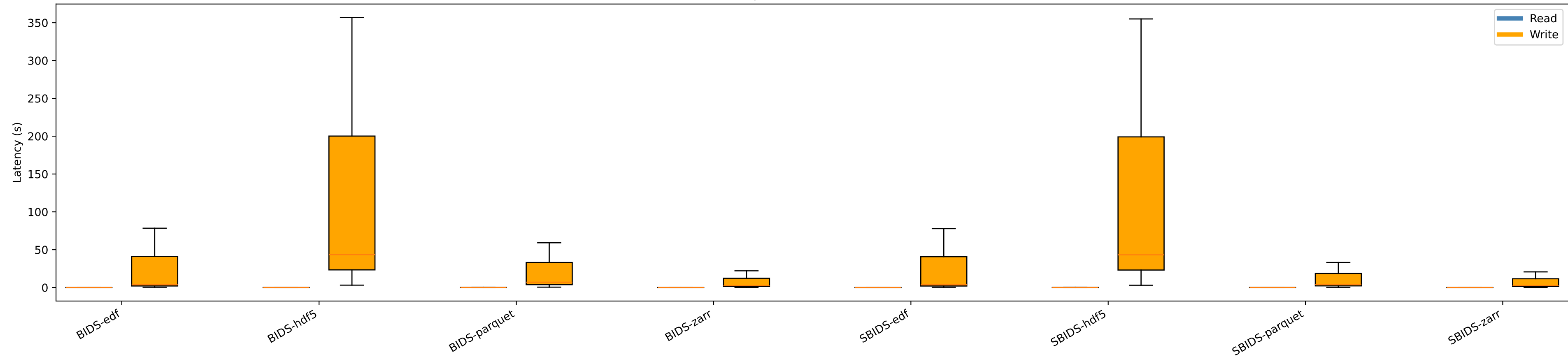
Read vs write latency (box) - Read window all channels (s)
