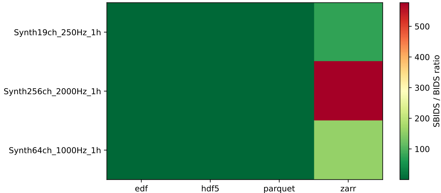
SBIDS vs BIDS speedup - Read throughput (bytes/s)
