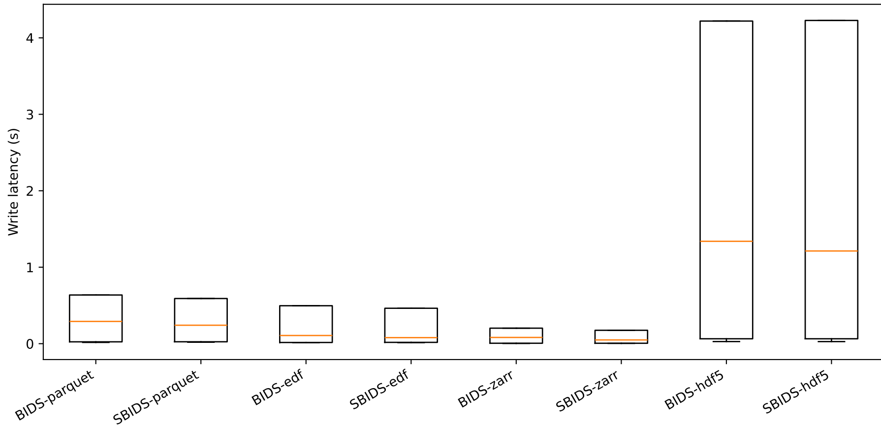
Experiment 2 - Write latency (s) (boxplots)
