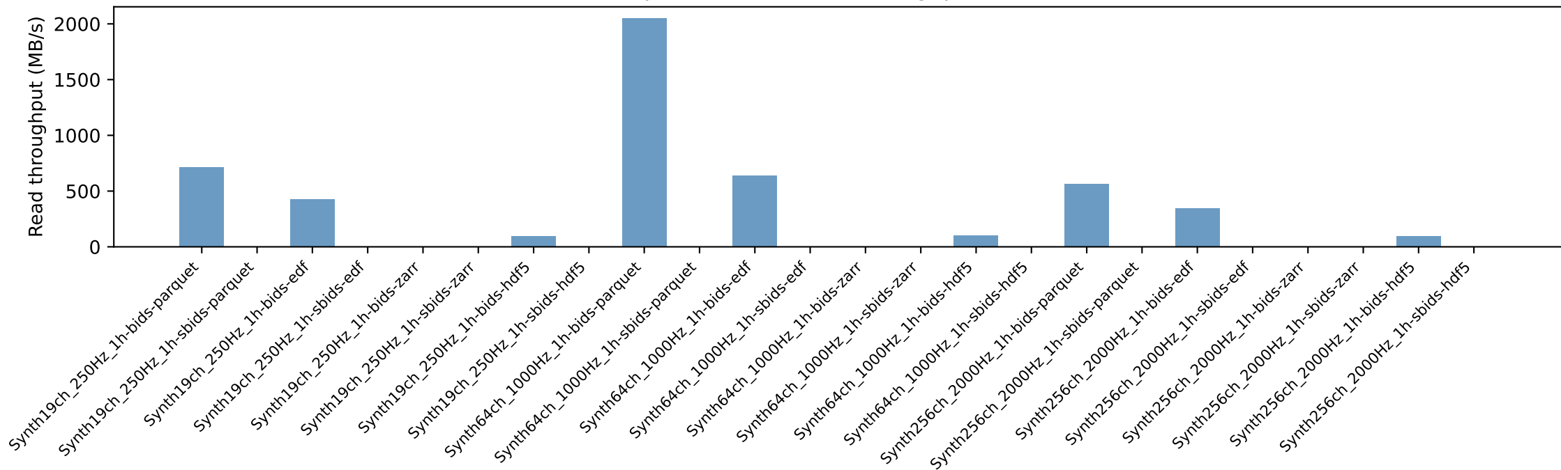
Experiment 2 - Read throughput (MB/s)
