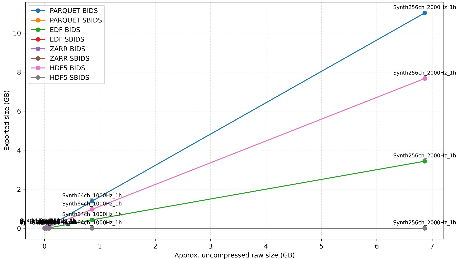
BIDS vs SBIDS size scaling across datasets (all)
