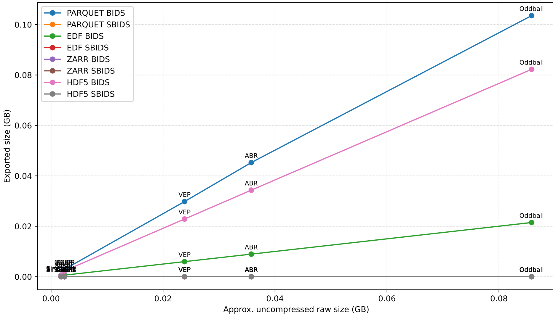
BIDS vs SBIDS size scaling across datasets (bin)
