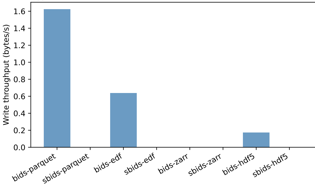
Synth Synth19ch_250Hz_1h - Write throughput (bytes/s)
