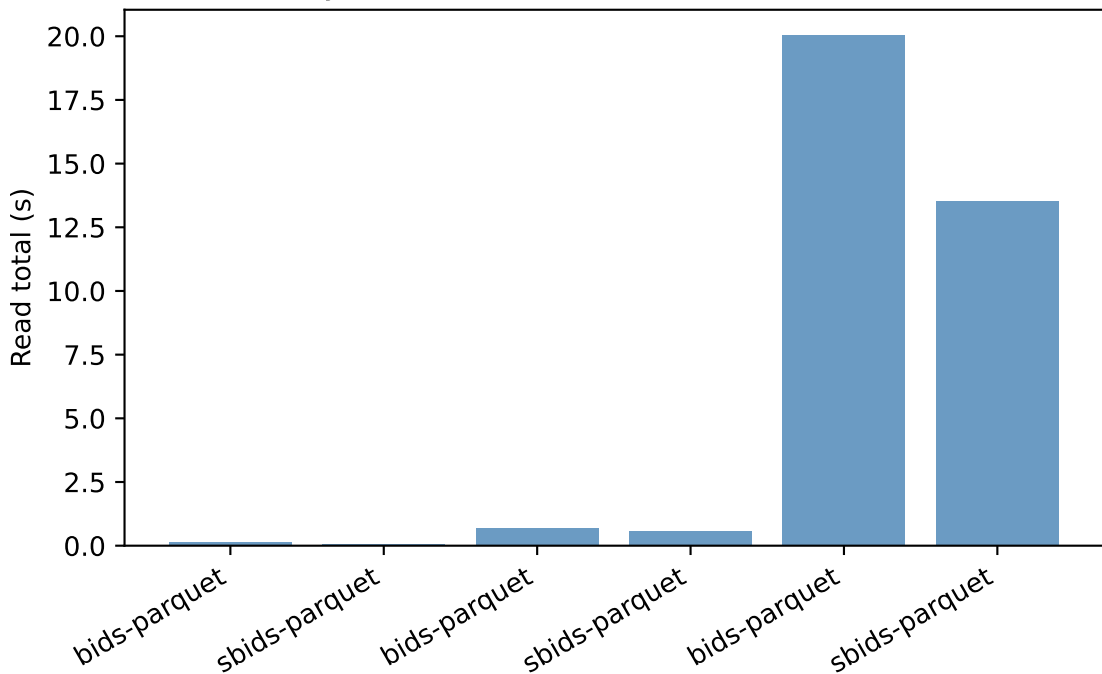
Synth format PARQUET - Read total (s)
