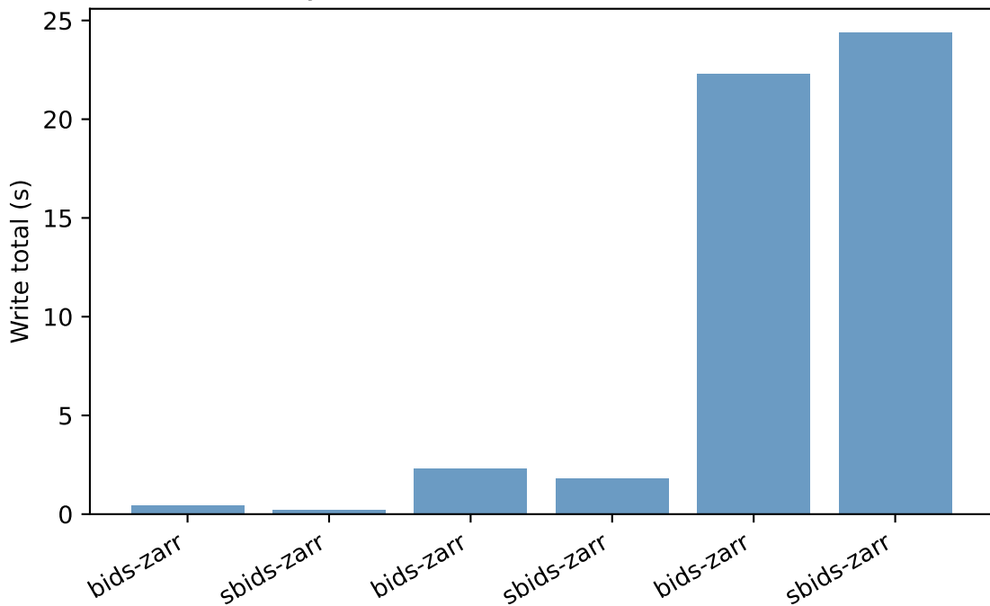
Synth format ZARR - Write total (s)
