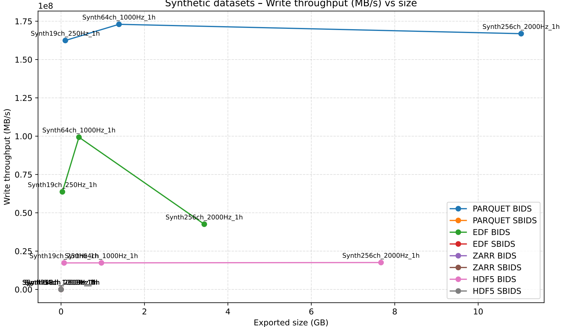
Synthetic datasets - Write throughput (MB/s) vs size
