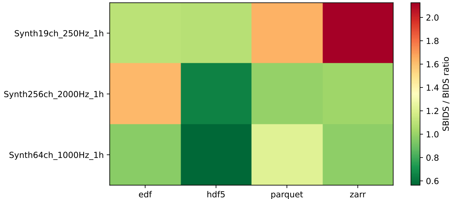
SBIDS vs BIDS speedup - Write throughput (bytes/s)
