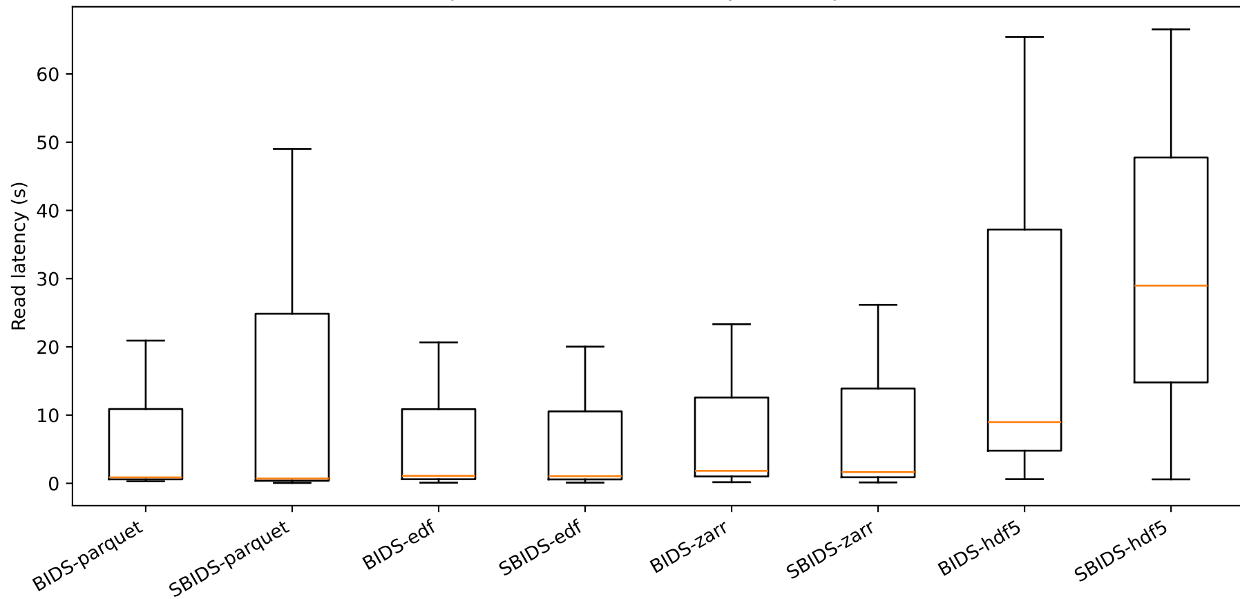
Experiment 2 - Read latency (s) (boxplots)
