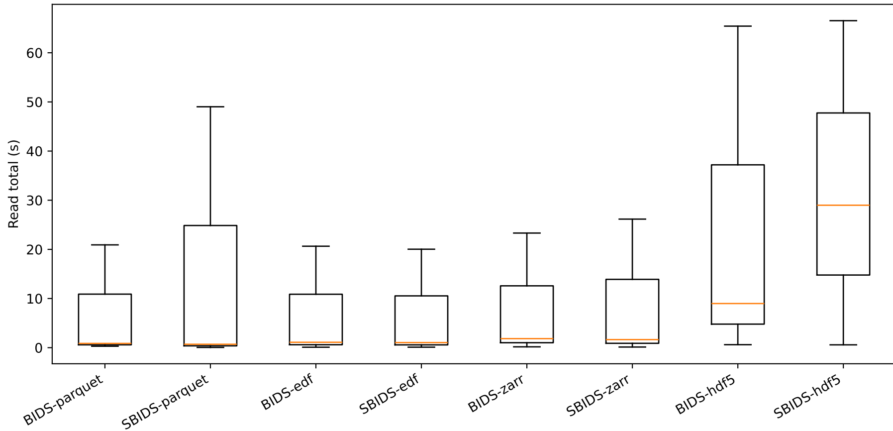
Experiment 2 - Read total (s) (boxplots)
