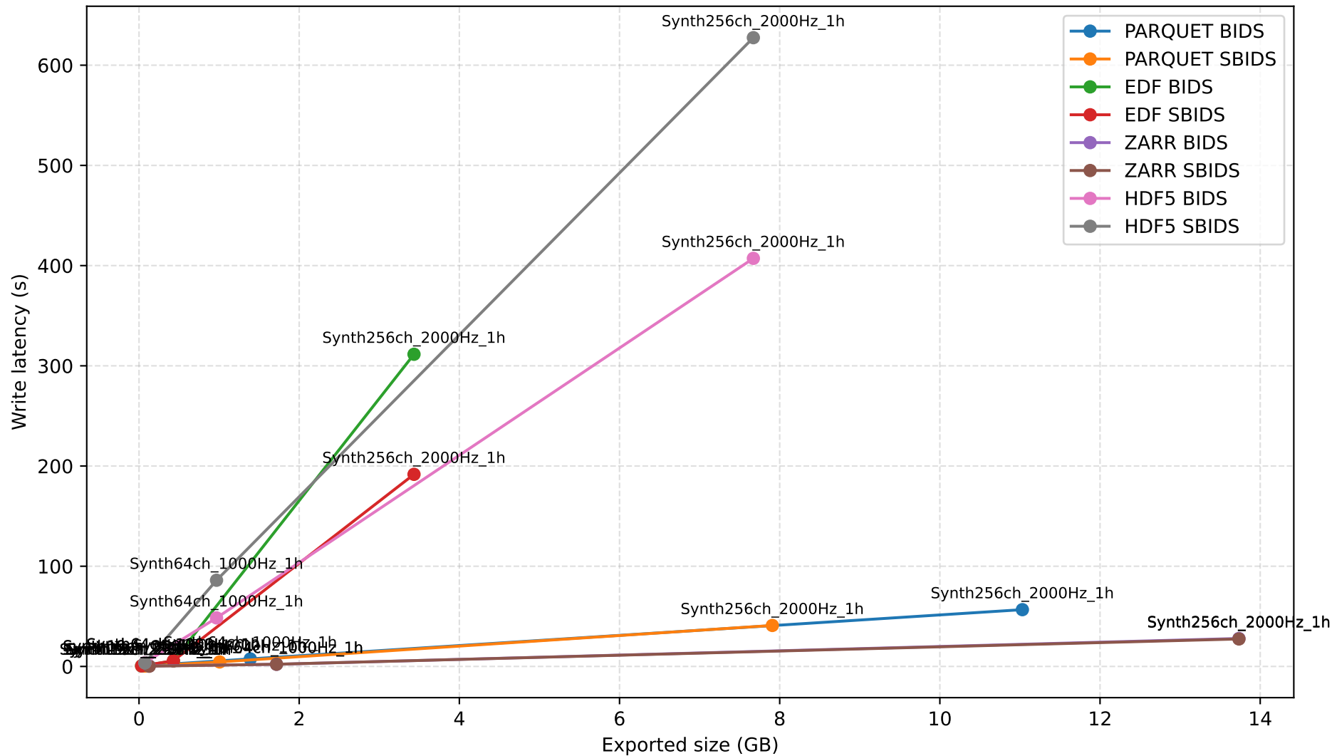
Synthetic datasets - Write latency (s) vs size
