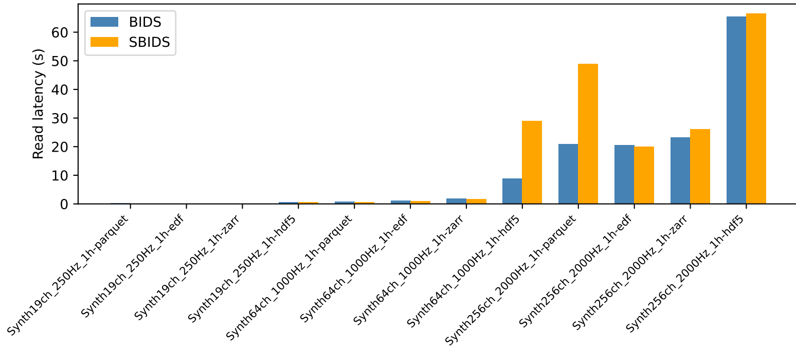
BIDS vs SBIDS - Read latency (s)
