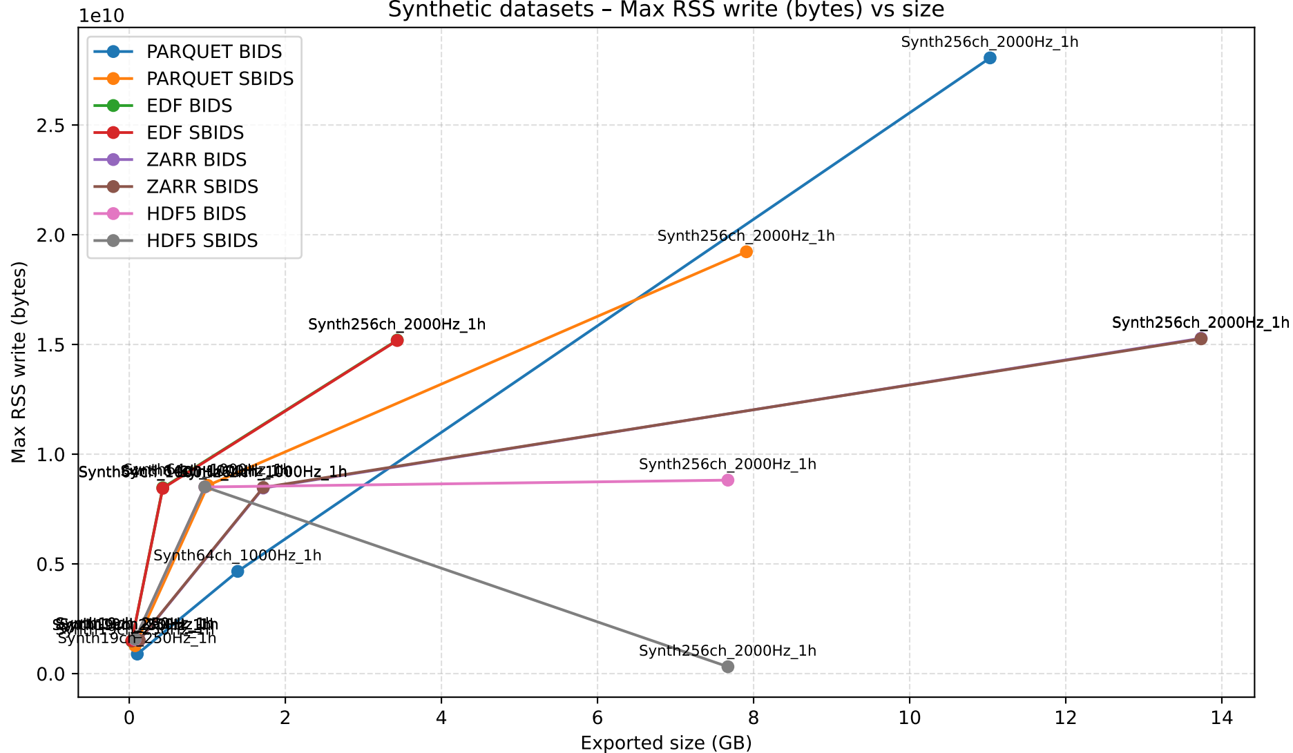
Synthetic datasets – Max RSS write (bytes) vs size
