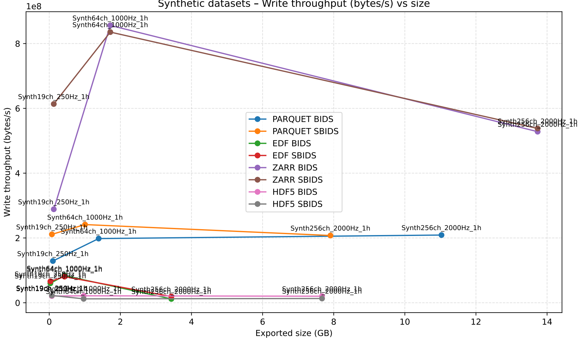
Synthetic datasets - Write throughput (bytes/s) vs size
