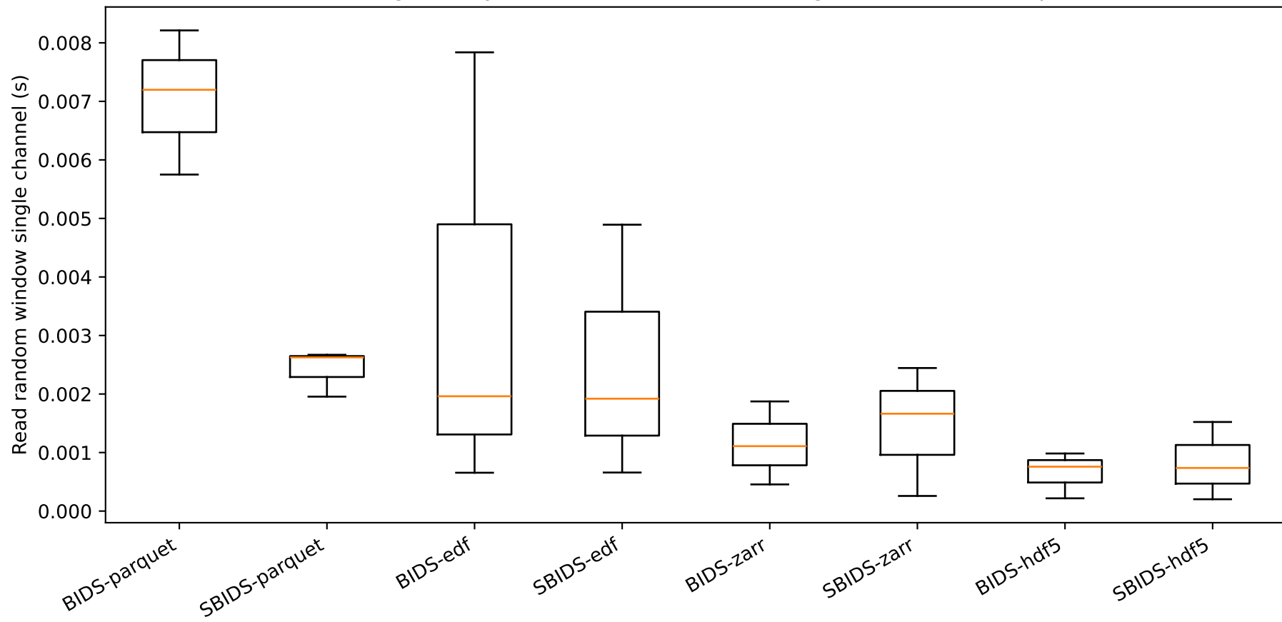
Streaming latency - Read random window single channel (s) (boxplots)
