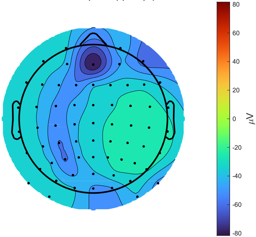
ASSR 40 Hz amplitude (spectopo)
