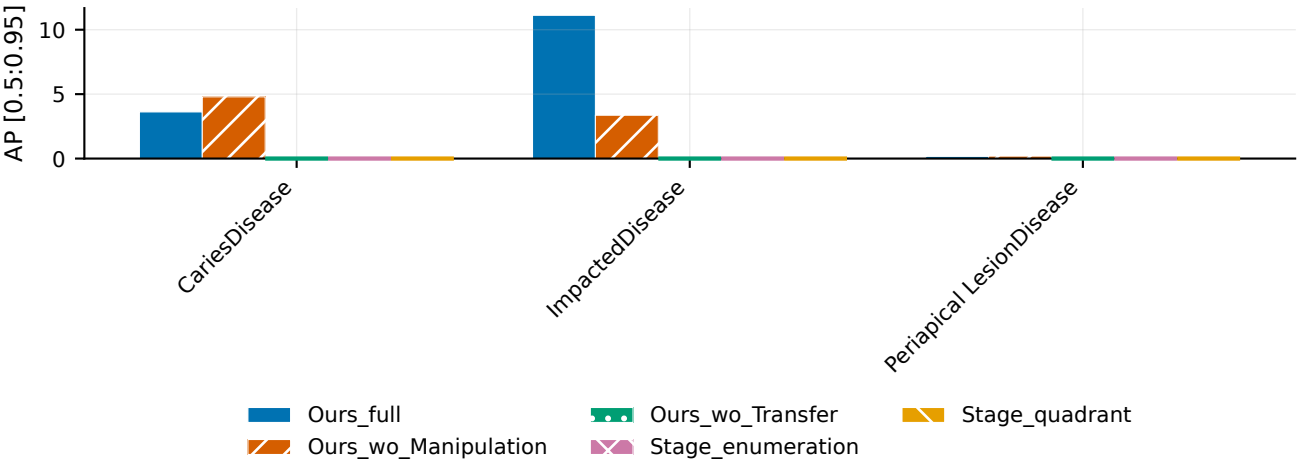
Per-class AP, diagnosis tier (our extension)
