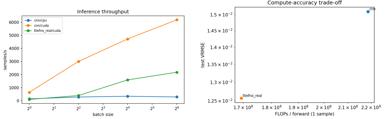
Figure 6: Left : Inference throughput (samples/s) on CPU and GPU (T4). Despite fewer FLOPs, LiteFNO is \sim 3\times slower on GPU (bs 64: 2,177 vs. 6,185 samples/s) due to FFT overhead at 32 \times 32 . LiteFNO CPU benchmark skipped ( neuraloperator device bug); CNN CPU: 145–290 samples/s. Right : VRMSE vs. FLOPs/forward. LiteFNO (0.0126, 169M FLOPs) sits on the better end of the compute–accuracy frontier than the CNN (0.0151, 219M FLOPs), yet has lower wall-clock throughput.
