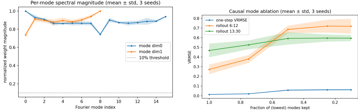
Figure 2: Left : Per-mode spectral weight magnitude (normalised), mean \pm std over 3 seeds. All modes exceed 74% of peak on both frequency axes; none fall below the 10% dead-mode threshold. The CP-factorised weights use their full spectral bandwidth, seed-robustly. Right : Causal mode ablation (3 seeds, mean \pm std). Keeping only the lowest-frequency fraction degrades one-step and rollout VRMSE immediately and monotonically; every mode is causally necessary.
