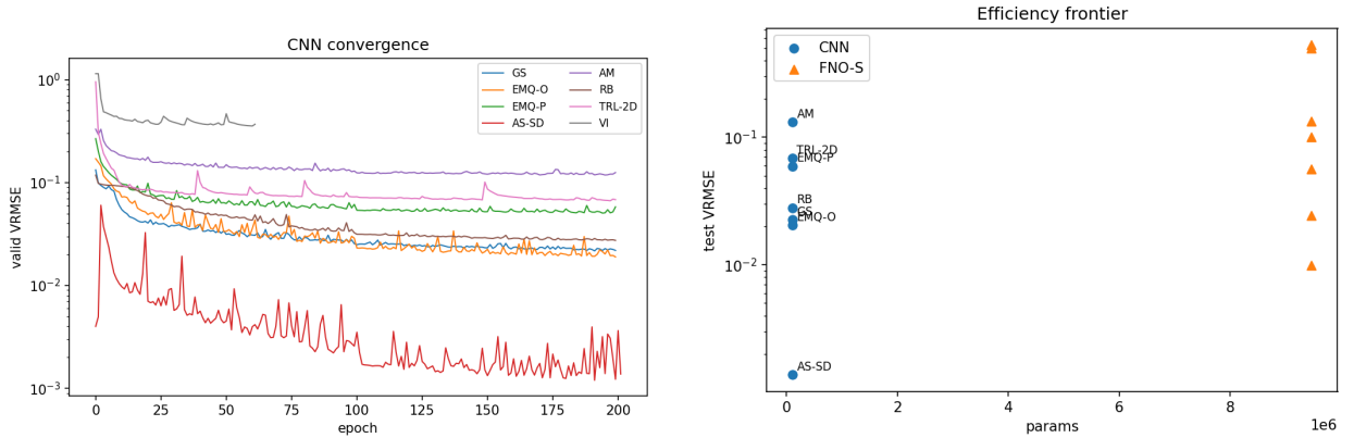
Figure 7: Left : Training-log VRMSE curves for the CNN arm across all 8 datasets (one line per dataset). Right : 8-dataset CNN vs. FNO-S accuracy scatter (log-VRMSE per dataset). These are dataset-level log summaries, not a two-arm matched-test comparison.
