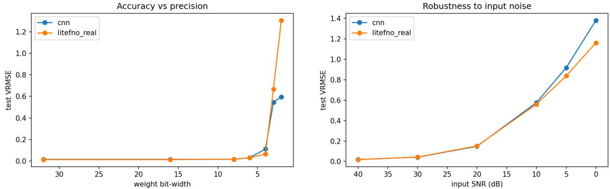
Figure 3: Left : VRMSE vs. numerical precision. Both models are lossless to int8 (CNN: 0.0151 \rightarrow 0.0160 ; LiteFNO: 0.0126 \rightarrow 0.0162 ); LiteFNO degrades more gracefully at int4 ( 0.064 vs. 0.111 ); both collapse at int3/int2. Model sizes: CNN 0.43 MB \rightarrow 0.108 MB (int8); LiteFNO 0.72 MB \rightarrow 0.180 MB (int8). Right : VRMSE vs. input SNR (dB). Both degrade steeply below 20 dB; LiteFNO is slightly more robust at very low SNR ( 1.163 vs. 1.382 at 0 dB).
