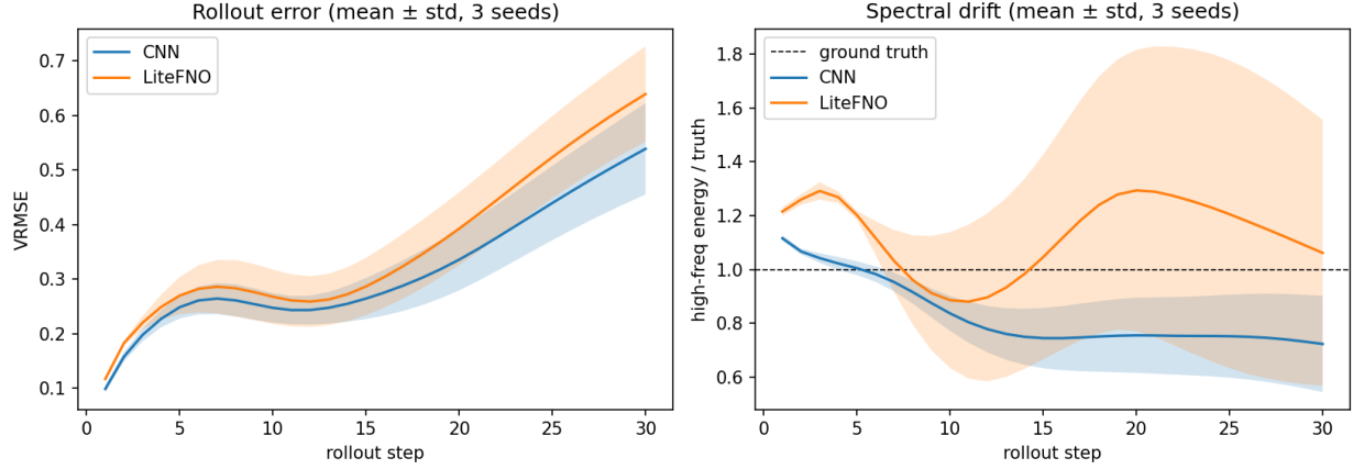
Figure 1: 3-seed rollout result (mean \pm std shading). Left : Autoregressive rollout VRMSE over 30 steps. The CNN accumulates error more slowly on average at both the 6:12 and 13:30 evaluation windows (step-30: 0.539 \pm 0.084 vs. 0.639 \pm 0.087 ). Right : High-frequency energy ratio (predicted / ground-truth). The CNN consistently over-smooths (ratio < 1 from step 5 onward). LiteFNO shows a transient over-sharpening peak around steps 2–5 followed by a return toward 1 and then descent; the high-freq ratio at step 30 is 1.06 \pm 0.51 (wide variance, seed-inconsistent). The spectral drift pattern is observable in individual seeds but not robust across seeds.
