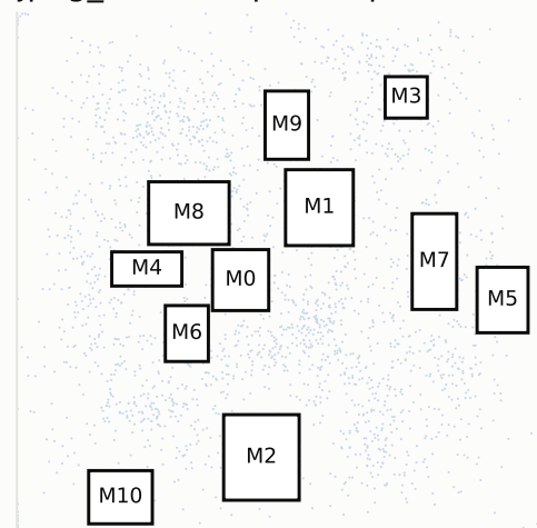
jpeg_like: floorplan + placement
