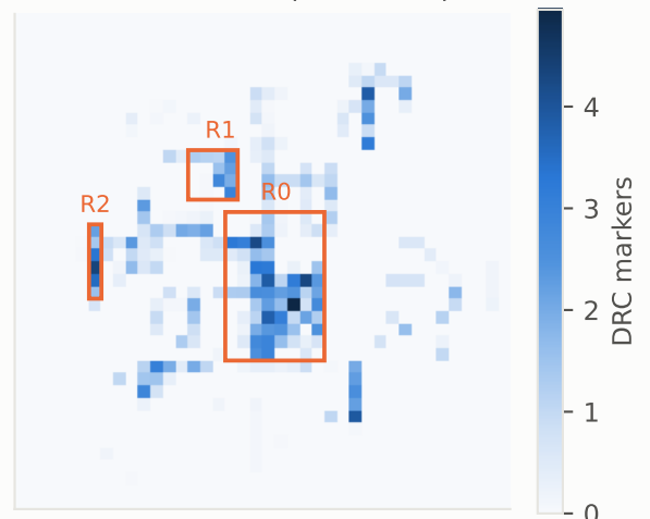
DRC markers (282 total)
