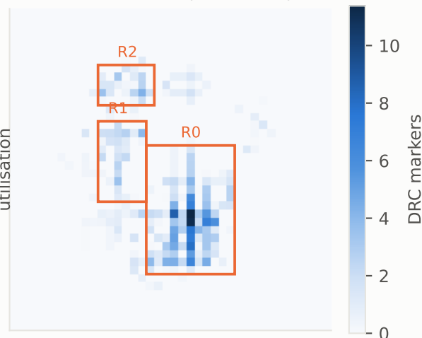
DRC markers (383 total)
