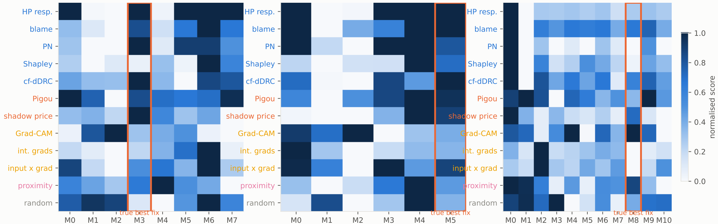
ibex_like: who is to blame?
