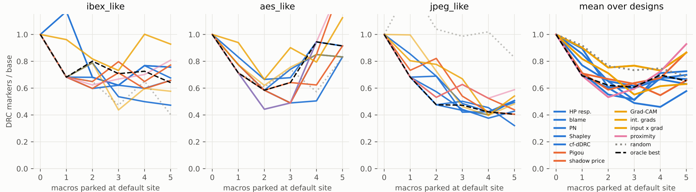
Park the accused: real place & route after removing the top-k blamed macros
