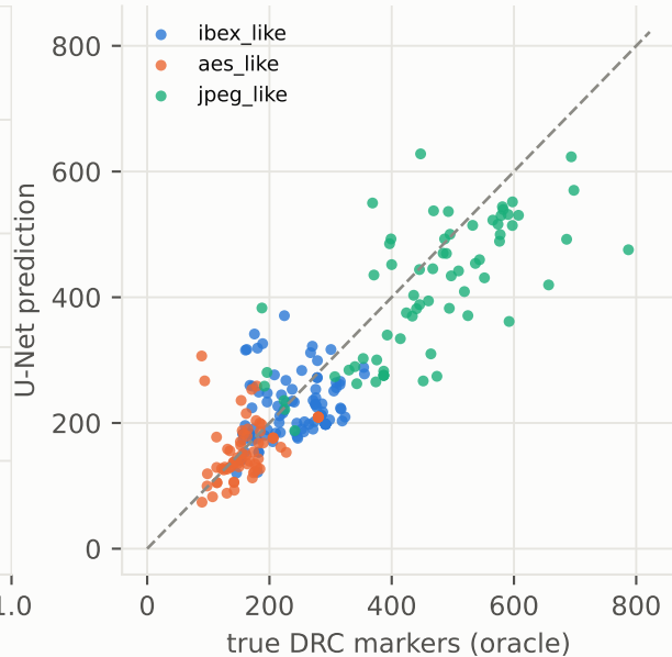
U-Net: held-out, mean rho = +0.51
