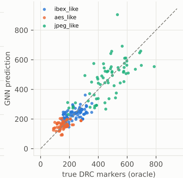
GNN: held-out, mean rho = +0.53
