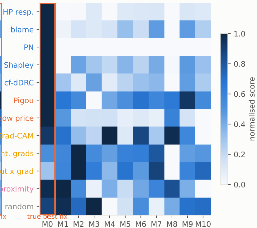
jpeg_like: who is to blame?
