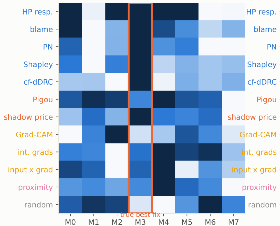
ibex_like: who is to blame?
