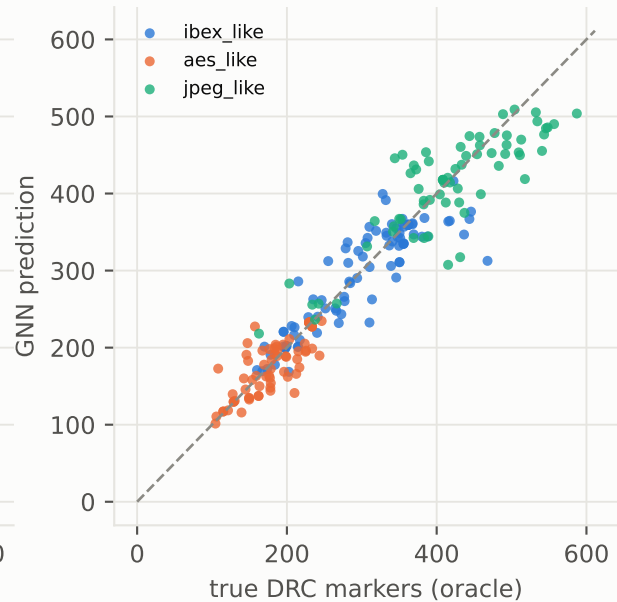
GNN: held-out, mean rho = +0.81
