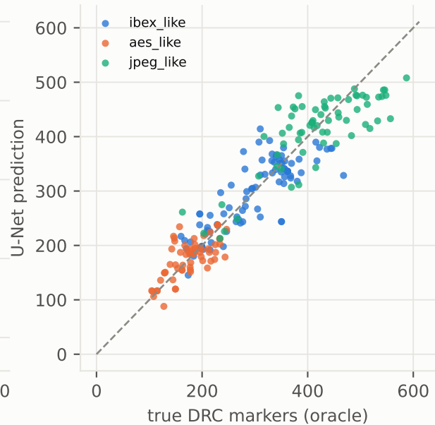
U-Net: held-out, mean rho = +0.72
