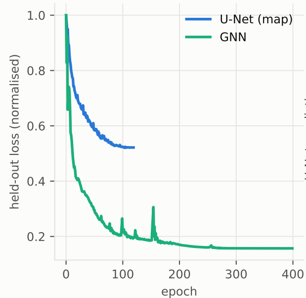
surrogate training
