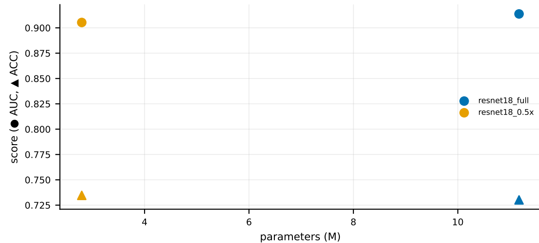
Accuracy vs size
