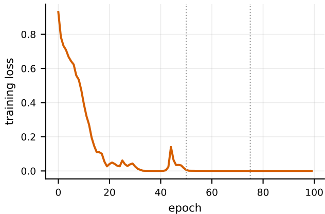
training loss
