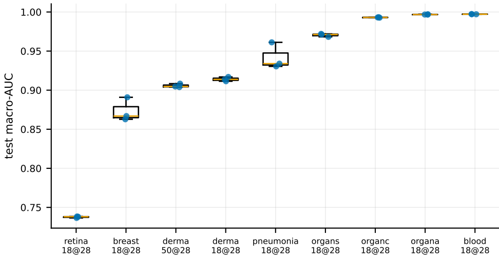
Test AUC across seeds (multi-seed datasets)
